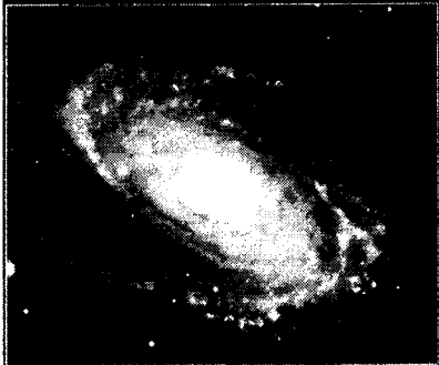
NGC3031 (spiral)
