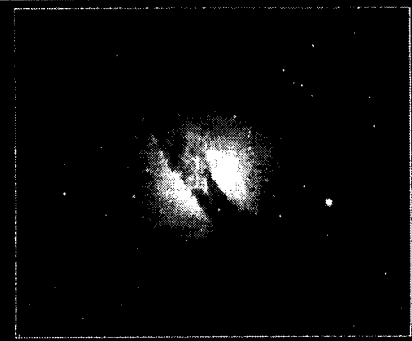
NGC5128 (elliptical)
